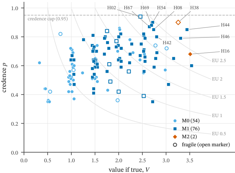
132 scored claims (median p = 0.64 ); labels: top 10 by EU
