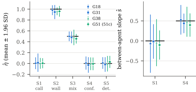
Second figure. Synthetic replies on the real schedules of G18, G31, G38 and G51c, with call starts jittered within their bounds. \hat{\eta} recovers 0, 1 and 0.5 (bias \leq 0.05 , power 1.0 against the wrong clock). Agent couplings correlated with cadence (S4) and detection loss (S5) do not move it. The estimator recovers the between-agent slope (S4: 0.5), with noise per period.
