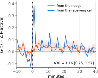
(a) #51 nudge → target (697)
