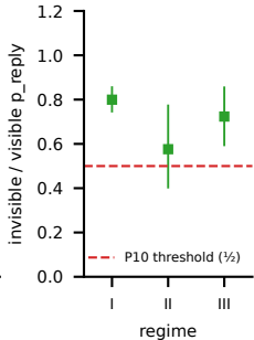
(b) placebo, replies
