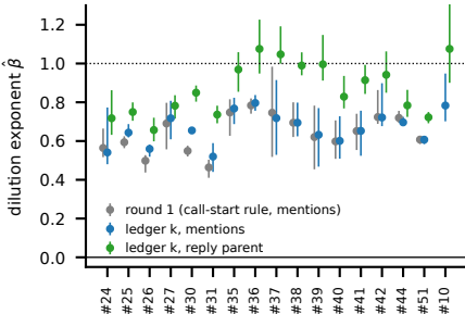
(a) per-period exponent
