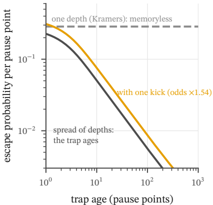
(a) aging vs Kramers (simulation)
