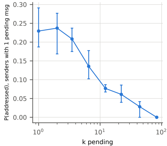
G27: \hat{\beta} = 0.69 [0.56, 0.80]
