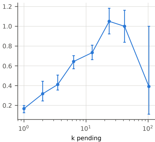
pending senders addressed per talk
