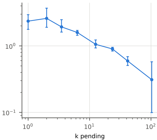
obs / exp under M_{\text{const}} (agentxday)
