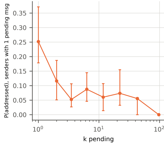
G39: \hat{\beta} = 0.62 [0.45, 0.78]
