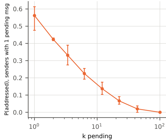
G44: \hat{\beta} = 0.72 [0.69, 0.76]
