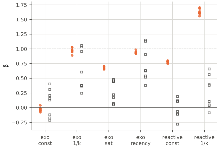
B Generative agents: D1 backlog (●) vs. D2 timer wakes, 300 s (□)
