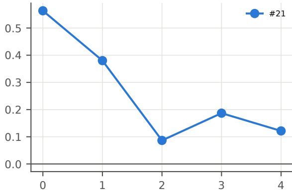
P4 polarization along \hat{g} (daily)
