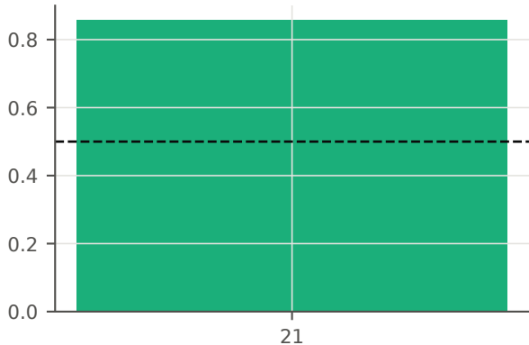
P9 \beta J_0/n (upper bound)
