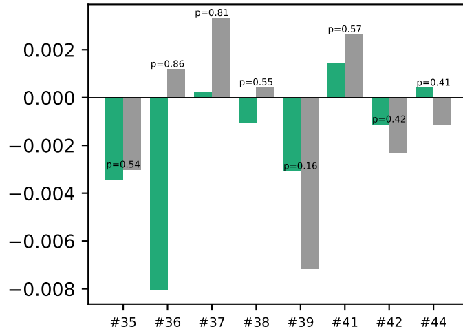
pair EP (nats/bin)
