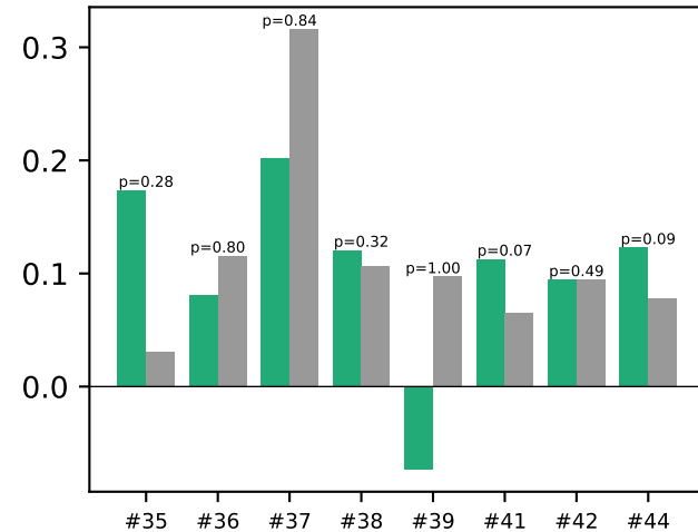
kinetic-Ising J_{\text{sym}}
