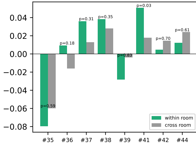
excess lagged corr \kappa
