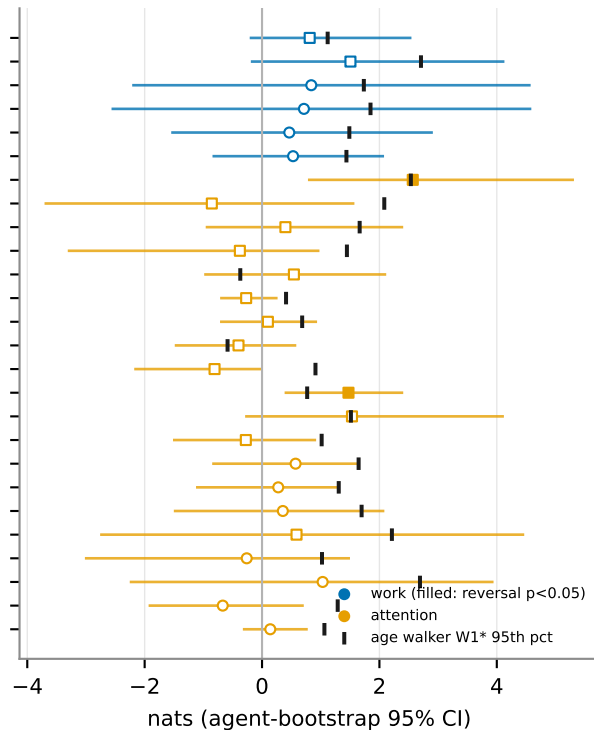
(b) rotation-summed cycle affinity A_{cyc}
