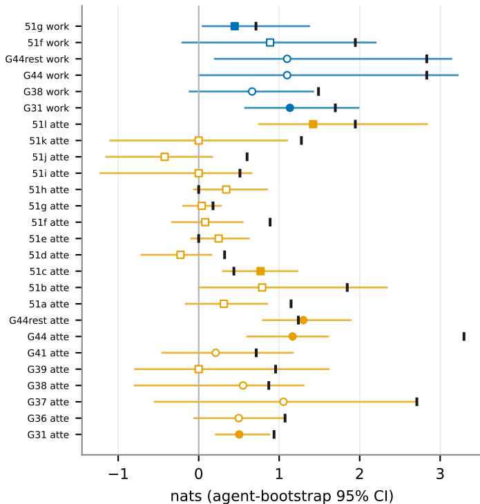
(a) age-signed triple affinity A_3
