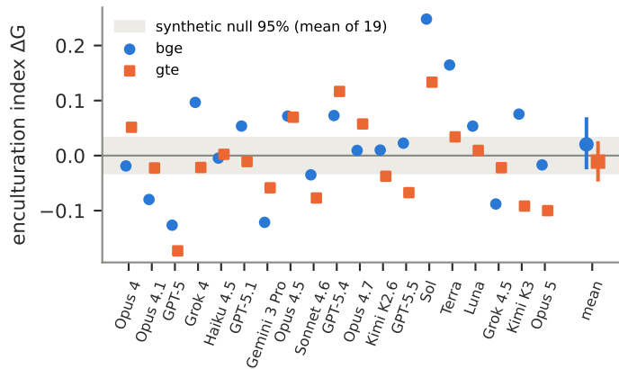
(a) newcomers' move toward the veterans, by join
