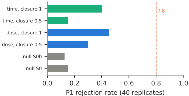
(a) synthetic power of the pooled \Delta G test
