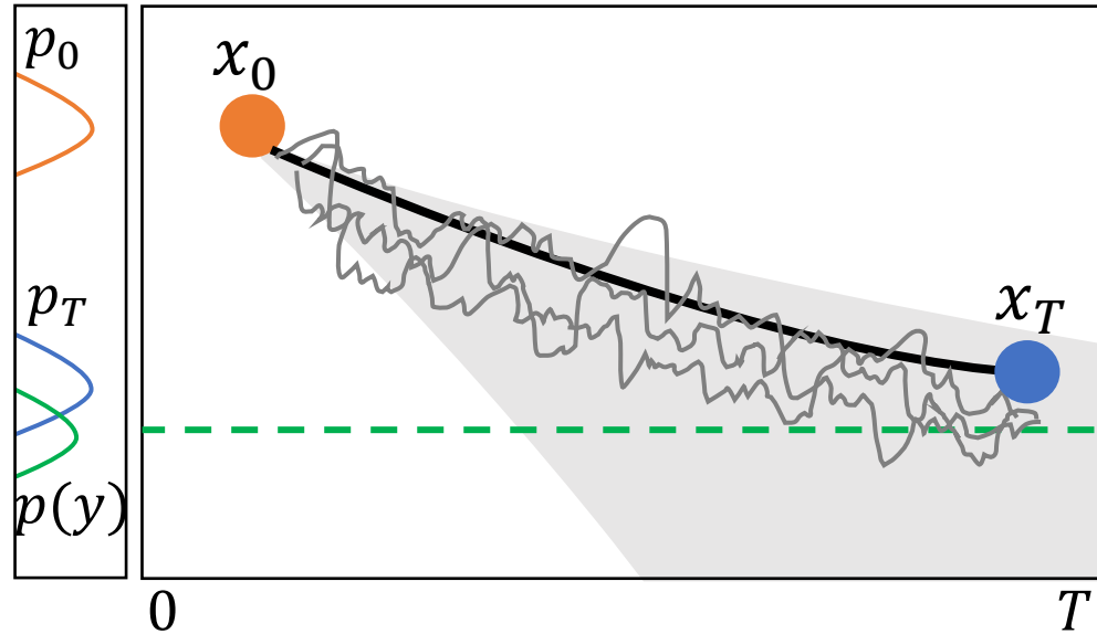
(a) Forward process of score-based diffusion model
