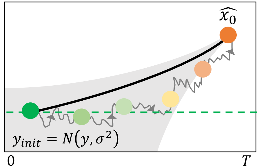
(b) Reverse process of score-based diffusion model
