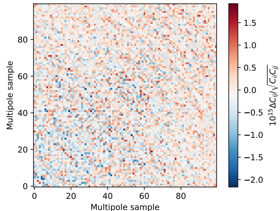
OneCov refinement versus the base grid
