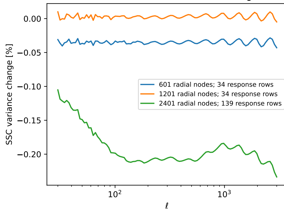
OneCov refinement versus the base grid
