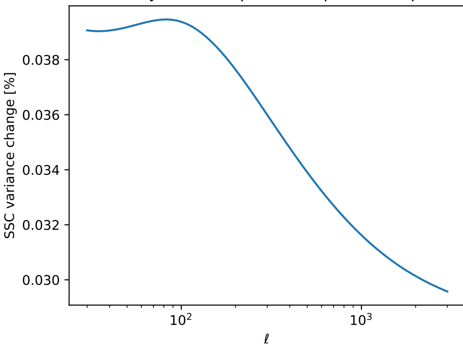
Analytic versus pixelized spherical cap
