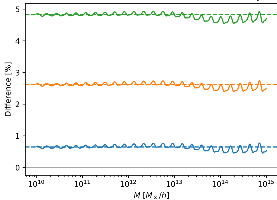
Native abundance; dashed = normalization only
