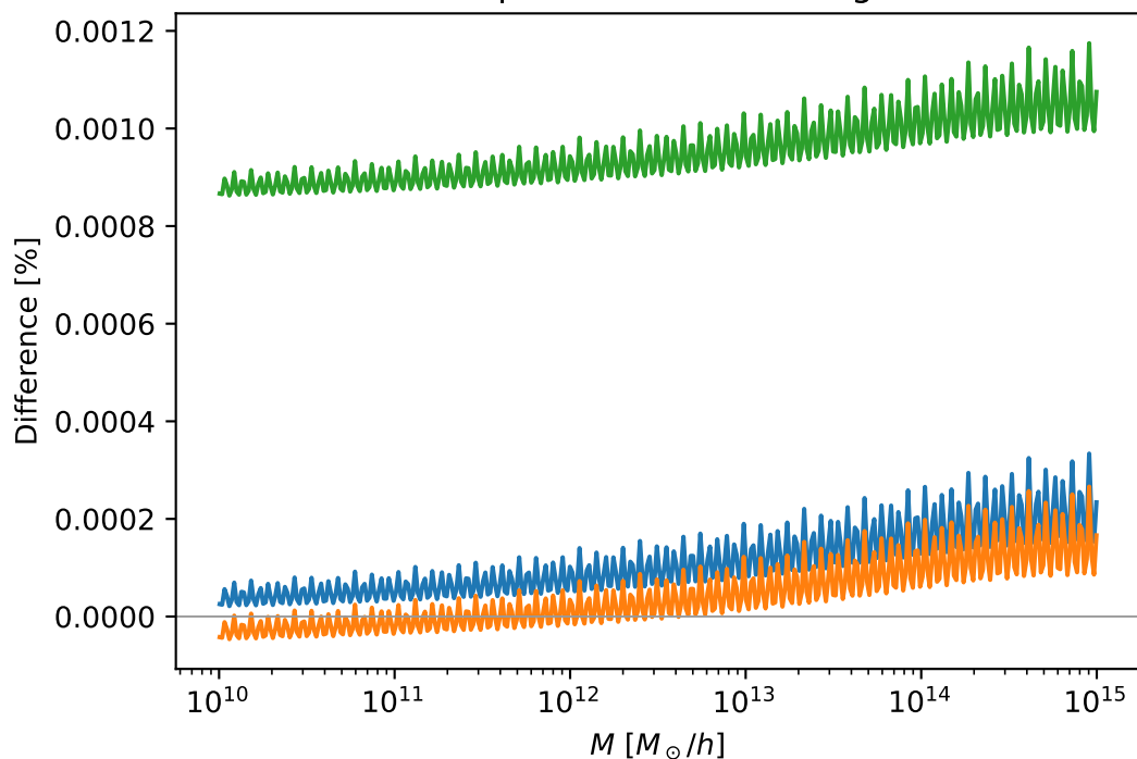
Abundance after removing normalization factor
