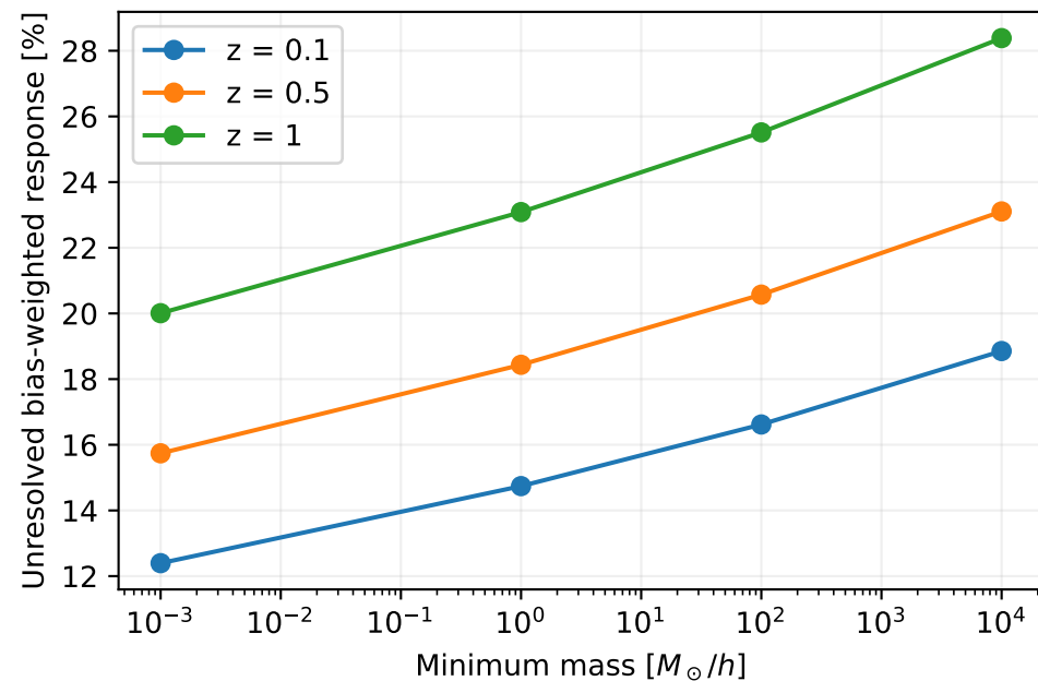
Lower halo-mass cutoff: unchanged fitted halo model Power beyond the supplied CAMB grid is log-log extrapolated
