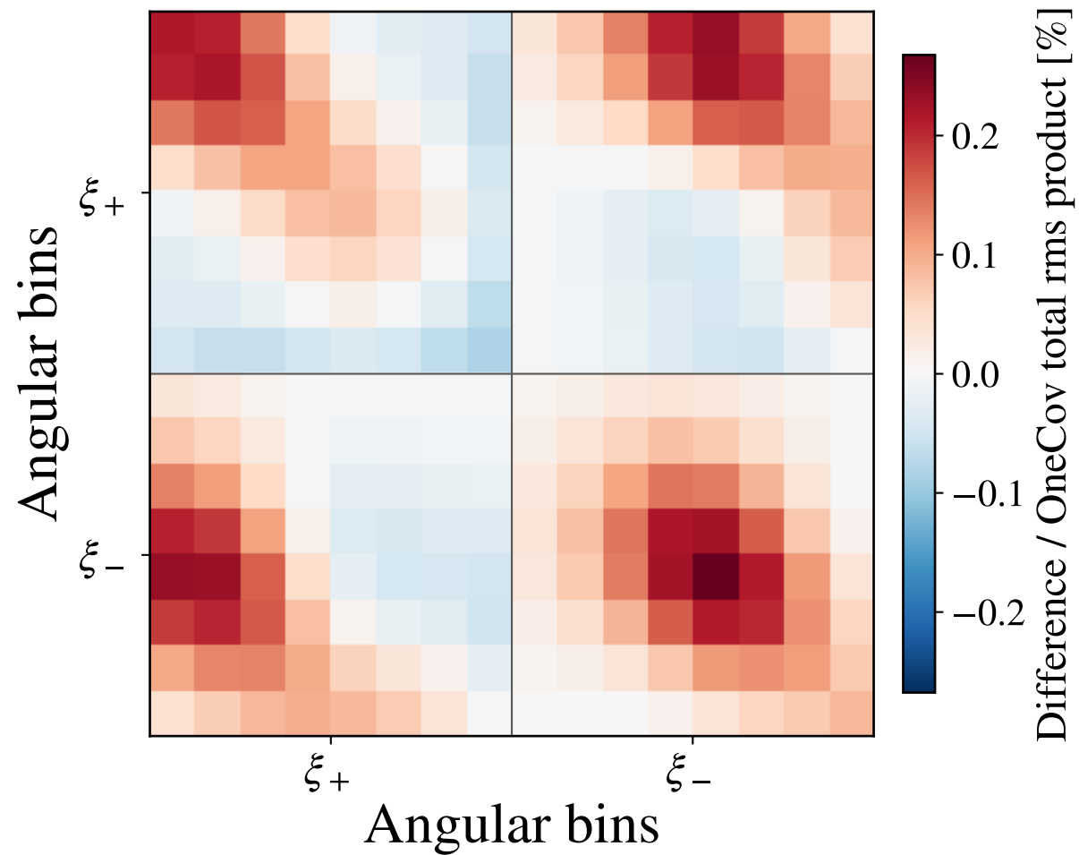
Connected non-Gaussian
