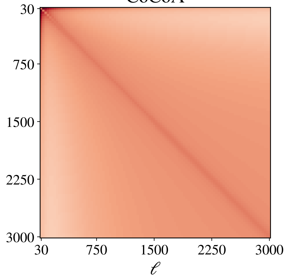
CoCoA
