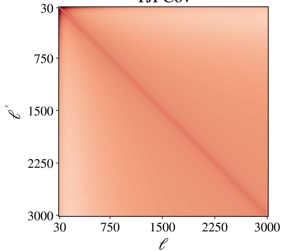
TJPCov
