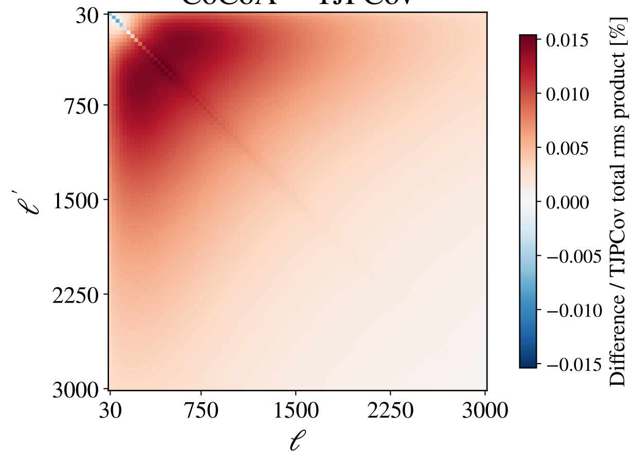
CoCoA – TJPCov
