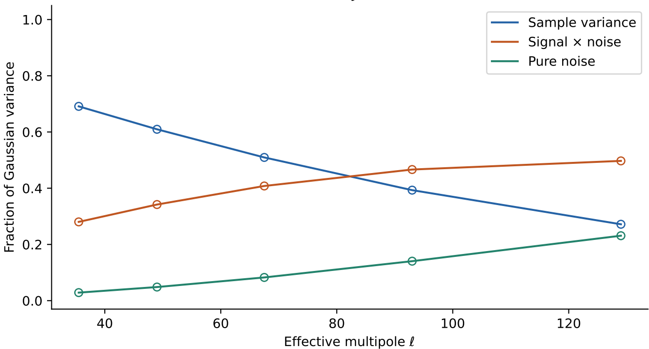
CoCoA lines / TJPCov markers
