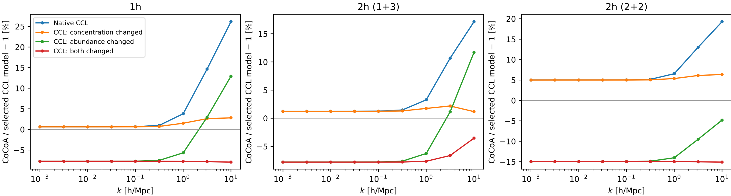
Public CCL fit switches at z=0.5 , equal k pairs Diagnostic models: matching fit names does not match normalization conventions
