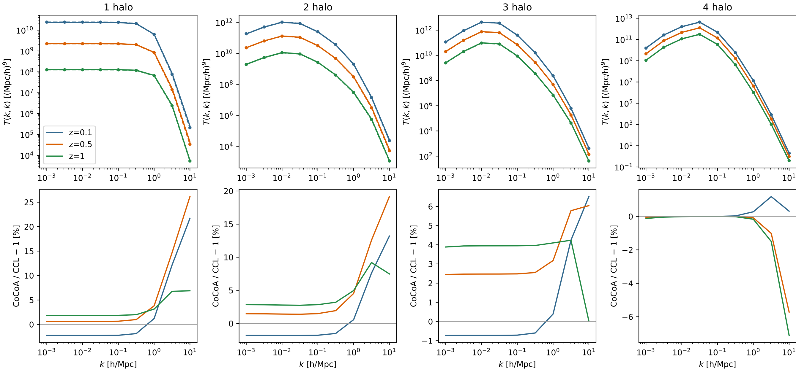
Matter trispectrum, equal k pairs · solid: CoCoA; dashed: TJPCov/CCL Native halo prescriptions, same CAMB inputs; no survey projection
