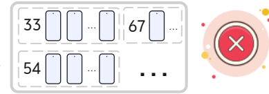
Wrong Traj.
