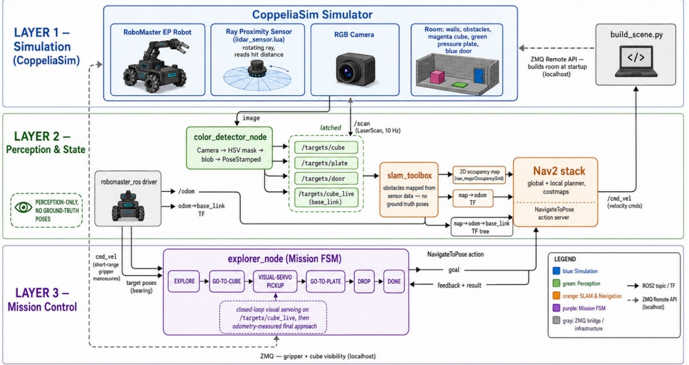
Fig. 2. System architecture in three layers: simulation (blue), perception and state estimation (green), and mission control (purple). Orange: Nav2 and slam_toolbox (third-party). Arrows show ROS 2 topics, TF transforms, and the ZMQ side-channel.
