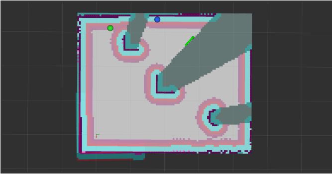
Fig. 4. Occupancy grid map built by slam_toolbox during exploration. White cells are free space, black cells are obstacles, and grey is unexplored. The planned path from Nav2 is shown in green.
