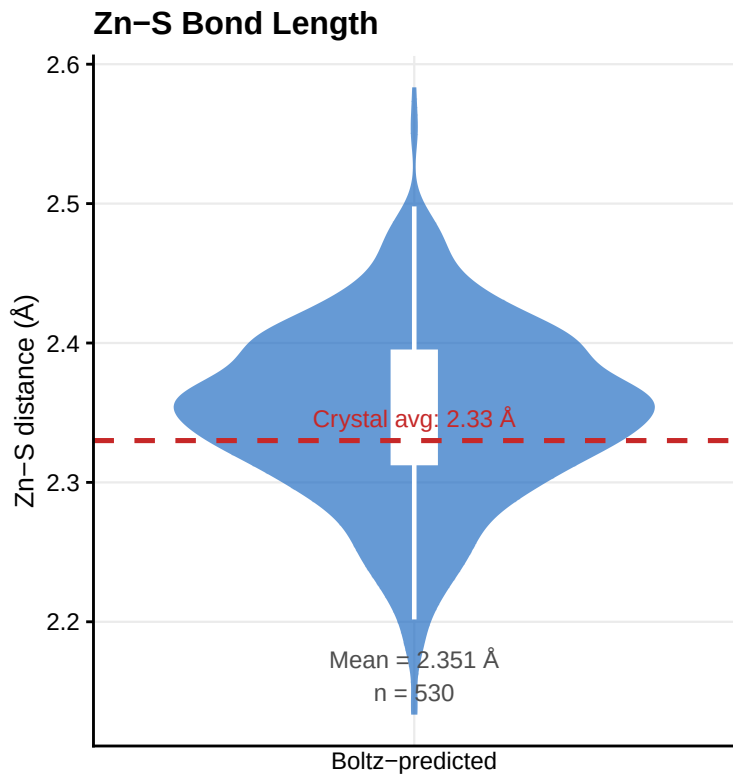
Figure 2 – Zn 2+ Coordination Geometry: Boltz Predictions vs Crystal Reference
