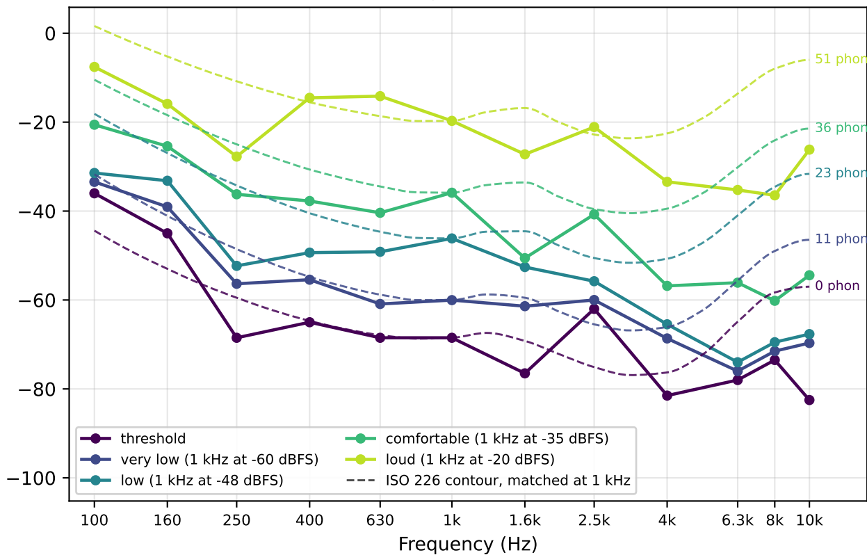
Measured equal-loudness curves
