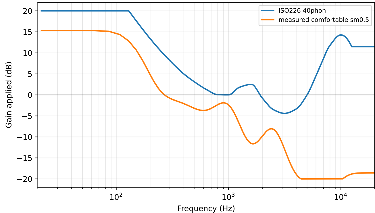
Equalizer gain curves: how much each frequency is boosted or cut
