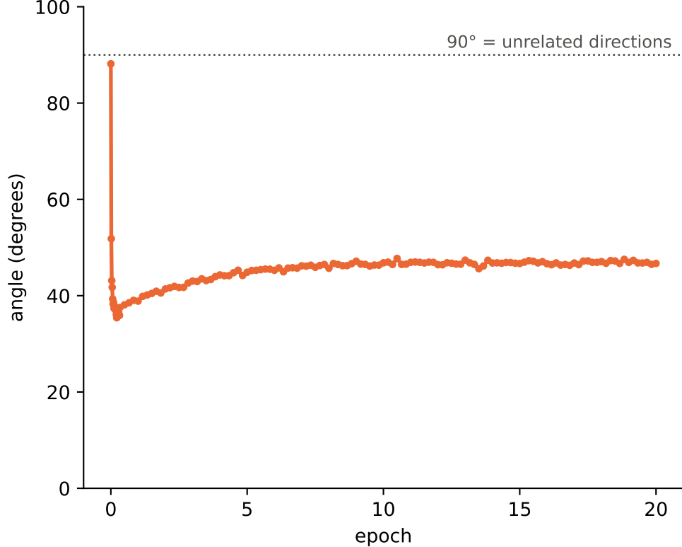
Angle between FA error signal and backprop error signal
