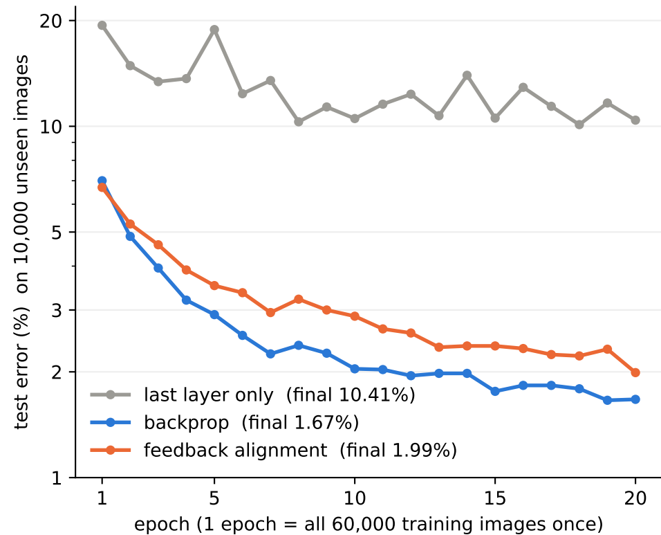
Test error during training
