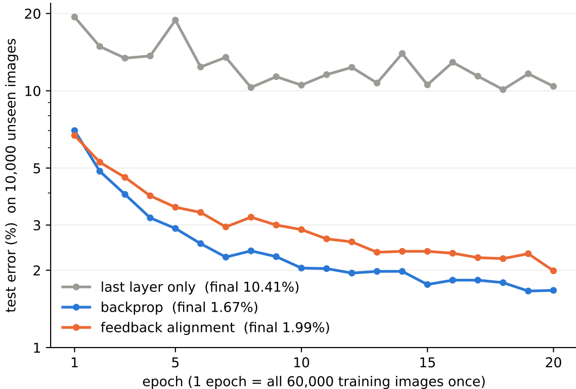
Test error during training
