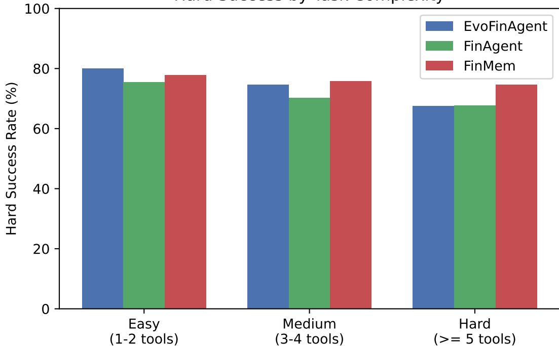
Hard Success by Task Complexity
