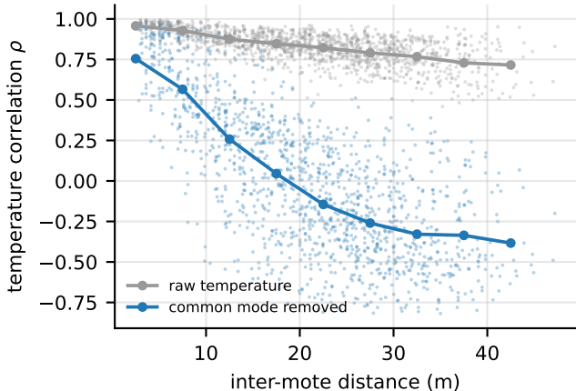
Spatial decay of correlation
