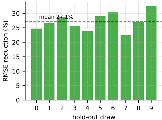
Gain from the graph term
