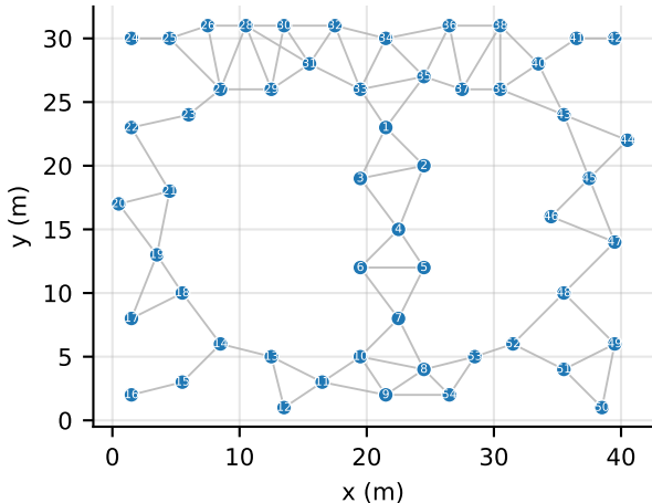
54 motes, A_\theta at 6 m radius (88 edges)
