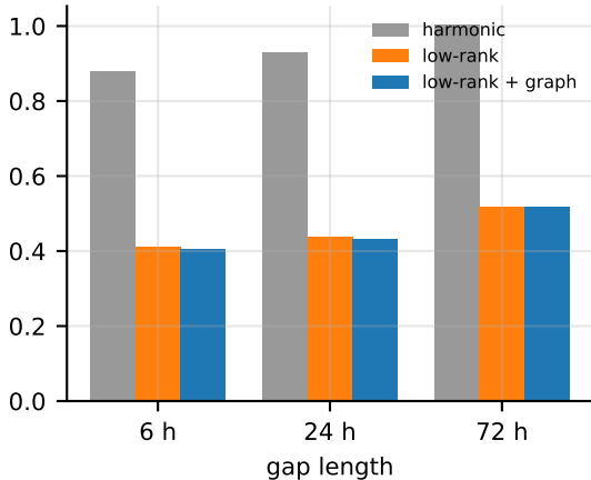
Long gaps: 61.7% of missing mass
