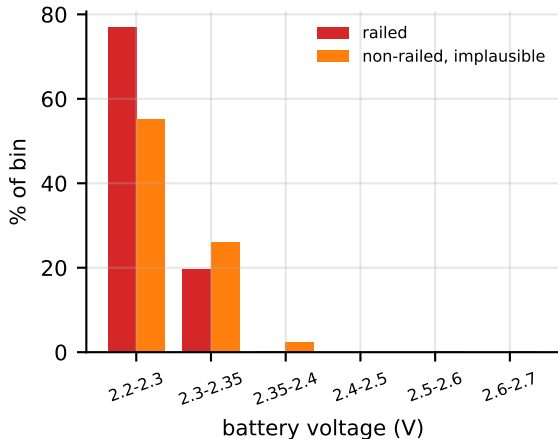
Two failure modes, separable
