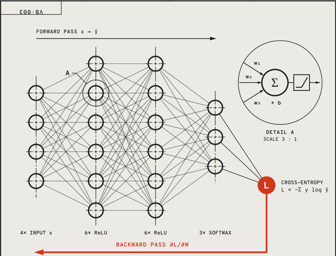
FIG. 1 MULTILAYER PERCEPTRON – FORWARD AND BACKWARD PASS
