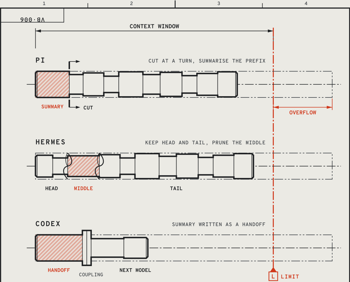
FIG. 1 ONE OVERFLOWING SESSION, THREE COMPACTIONS – CUT, BREAK, HANDOFF
