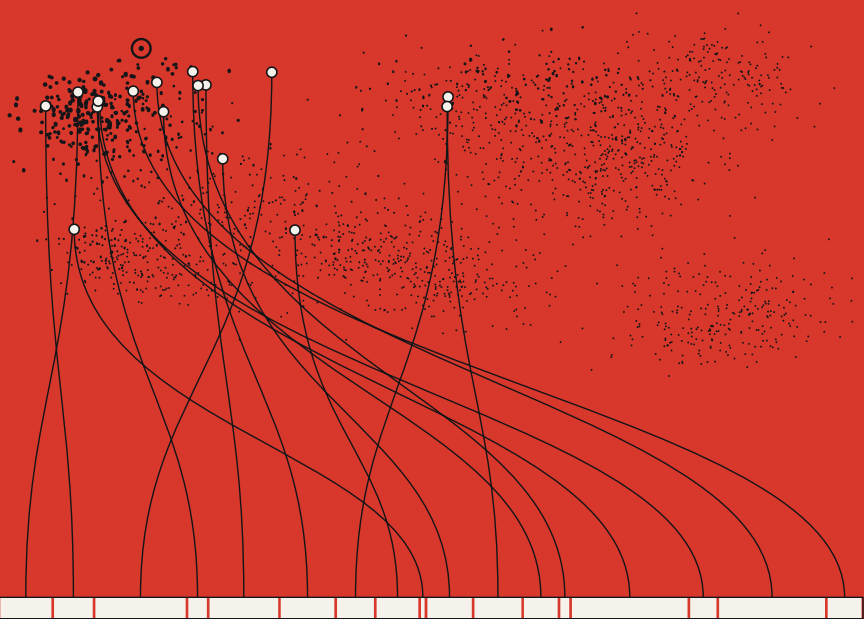
FIG. 0 2,400 document chunks in a 48-dimensional embedding space, flattened here by PCA; Q is the query. Maximal marginal relevance ( \lambda = 0.55 ) picks the 17 that fill an 8,192-token window (8,190 used), laid out most-relevant-at-the-ends. The chosen are in white.
