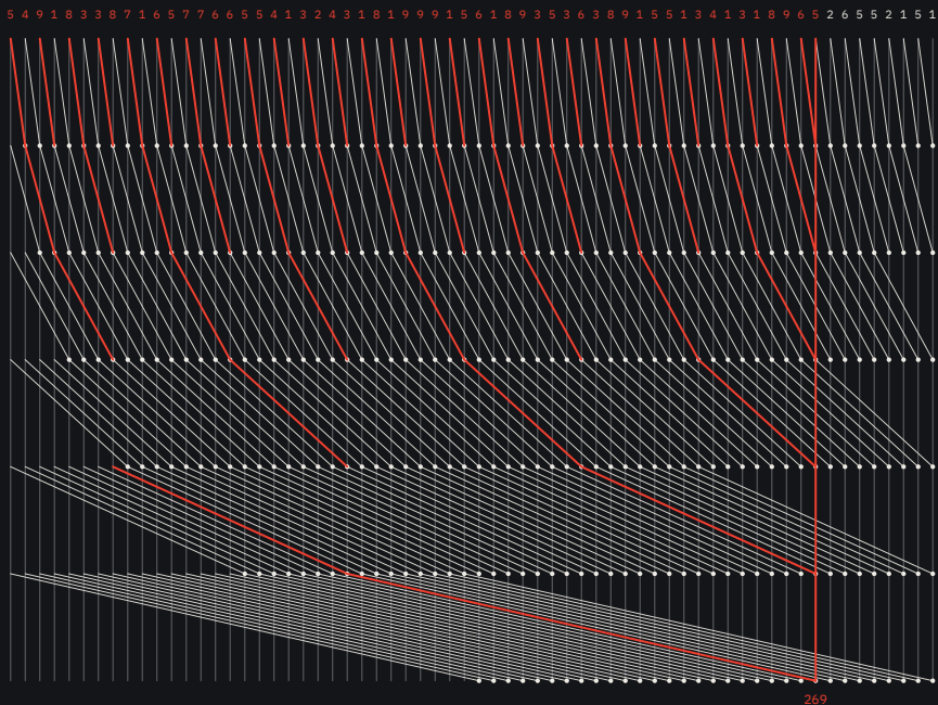
FIG. 0 A Kogge-Stone prefix sum, the pattern inside warp-level scans: 64 GPU lanes, 6 steps, 321 additions. At step k each lane adds the partial sum 2^k lanes to its left. In red: the additions lane 55 depends on, gathering 56 of the digits above into 269.
