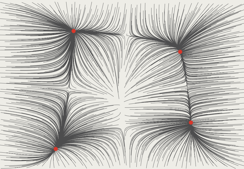
FIG. 0 Gradient descent ( \eta = 0.0006 ) from 1,472 starting points on Himmelblau's function, f(x,y) = (x^2+y-11)^2 + (x+y^2-7)^2 . 503,898 steps in all; every path ends in one of its 4 minima, in red.
