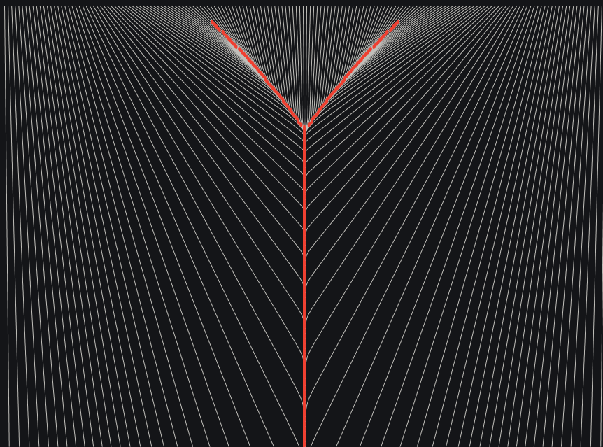
FIG. 0 Burgers' equation, u_t + u \cdot u_x = (0.01/\pi) \cdot u_{xx} – the classic benchmark for physics-informed networks – solved in this page by finite volumes (400 cells, 984 time steps). Lines: 170 fluid particles carried by the flow, time running down; red: shocks, where they collide.
