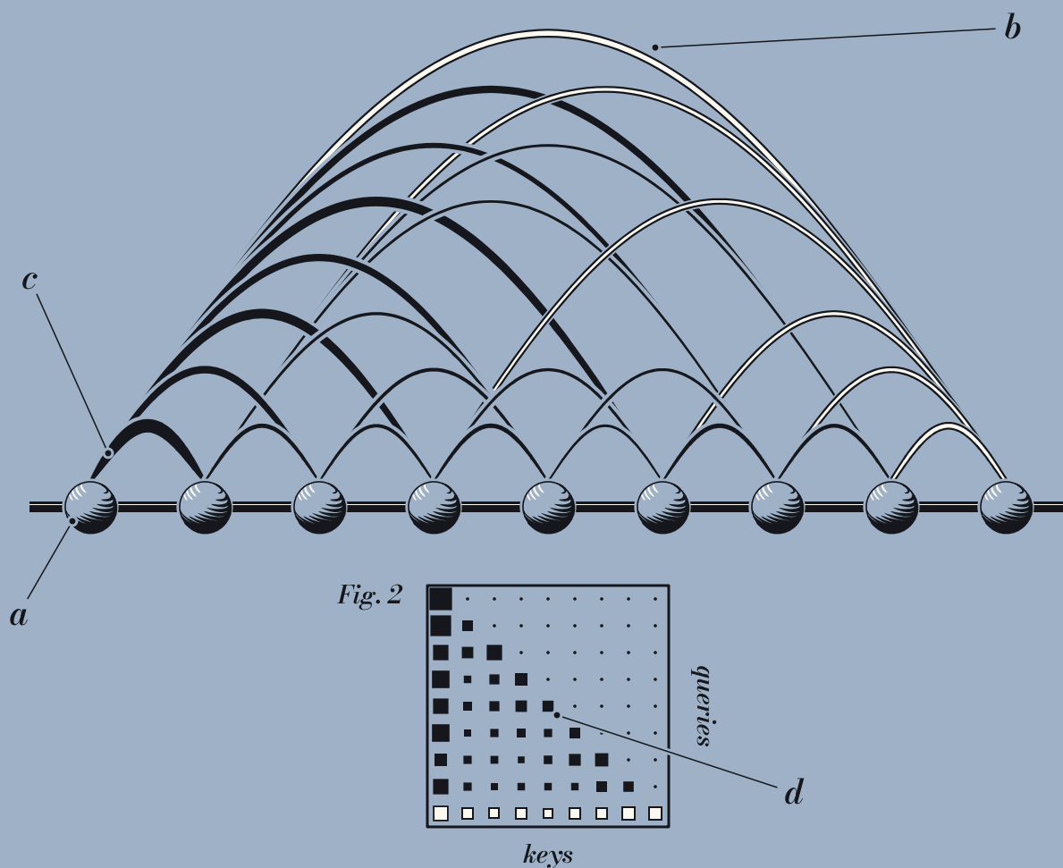
Fig. 1. One causal attention head over nine tokens, each arch weighted by \text{softmax}(QK^T/\sqrt{d}) . a tokens; b the last query, in white; c the attention sink. Fig. 2. The weights as a matrix; d its diagonal.
