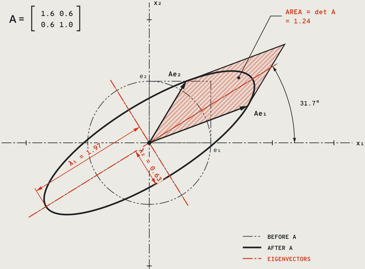
FIG. 1 A MATRIX IS A TRANSFORMATION – THE UNIT CIRCLE UNDER A
