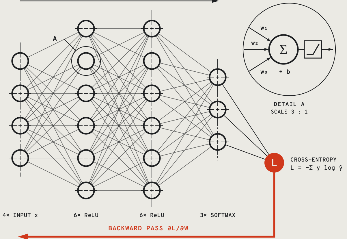
FIG. 1 MULTILAYER PERCEPTRON — FORWARD AND BACKWARD PASS
