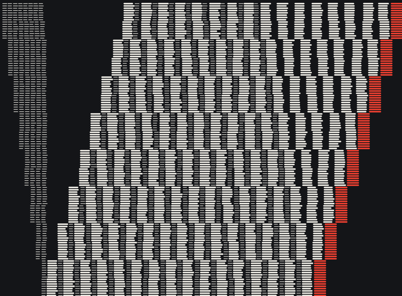
FIG. 0 One training step on a 128-GPU mesh – data 2 × pipeline 8 × tensor 2 × context 2 × expert 2 – simulated under a 1F1B schedule of 16 micro-batches with ±7% kernel-time noise. Each row is a GPU: thin = forward, thick = backward, red = gradient all-reduce.
