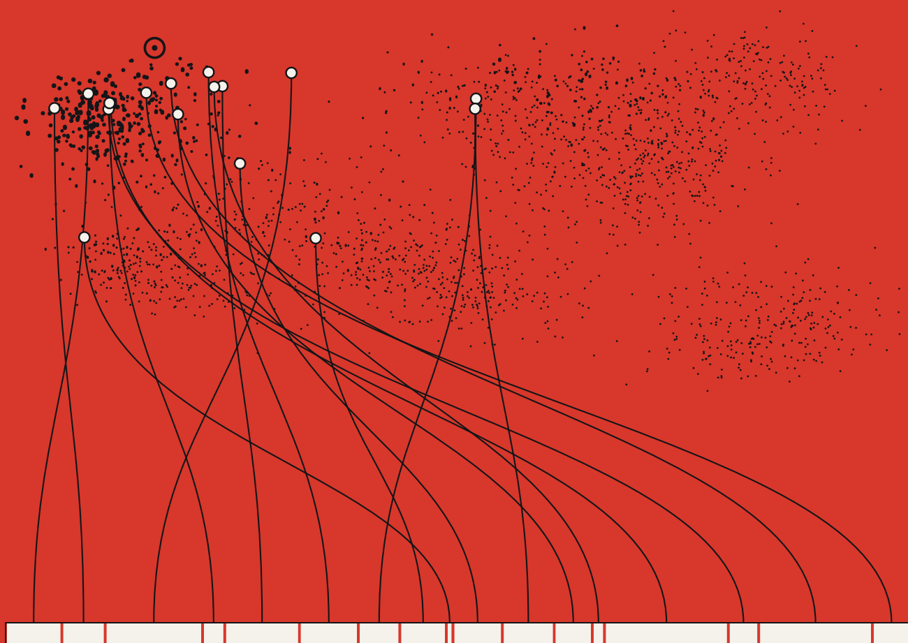
FIG. 0 2,400 synthetic document chunks in a 48-dimensional embedding space, flattened here by PCA; Q is the query. Maximal marginal relevance ( \lambda = 0.55 ) picks the 17 that fill an 8,192-token window (8,190 used), laid out most-relevant-at-the-ends. The chosen are in white.
