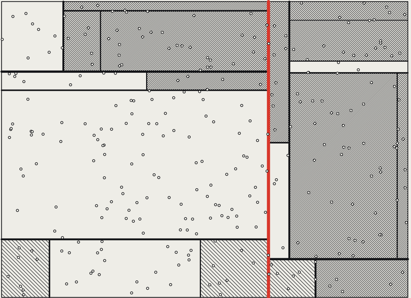
FIG. 0 A classification tree grown in this page by CART – Gini impurity, depth \leq 7 – on 300 labelled points of three classes. Every line is one question the tree asks, heavier the earlier it is asked; the first is red. 18 questions, 19 leaves, shaded by the class they vote for.
