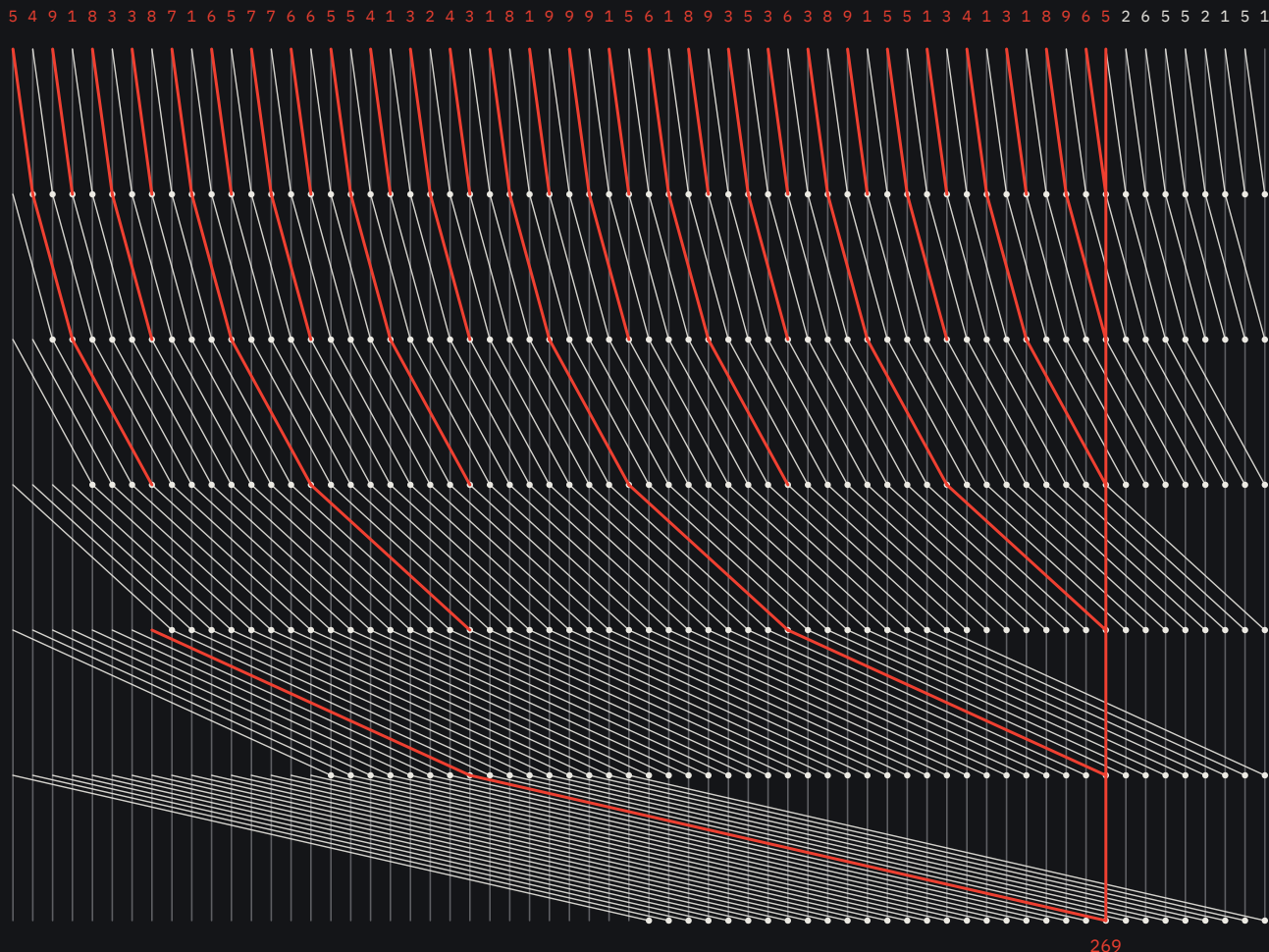
FIG. 0 A Kogge-Stone prefix sum, the pattern inside GPU scan kernels: 64 threads, 6 steps, 321 additions. At step k each thread adds the partial sum 2^k places to its left. In red: the additions thread 55 depends on, gathering 56 of the digits above into 269.
